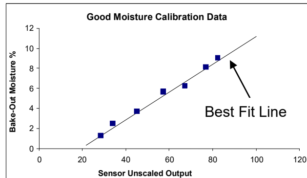
Figure 17: Example of Good Material Calibration
