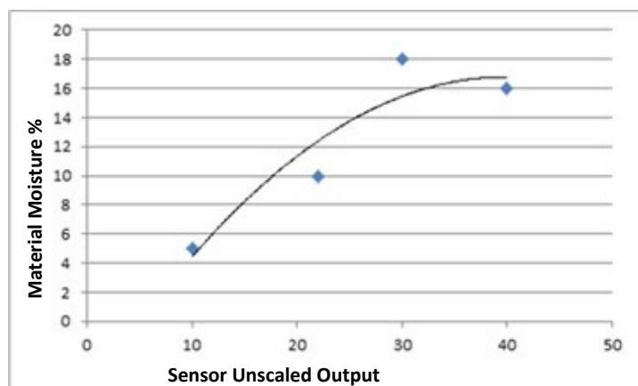
Figure 20: Example of a Bad Quadratic Calibration
