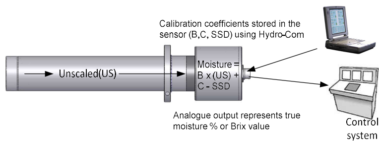
Figure 21: Calibration inside the Hydro-Probe SE
