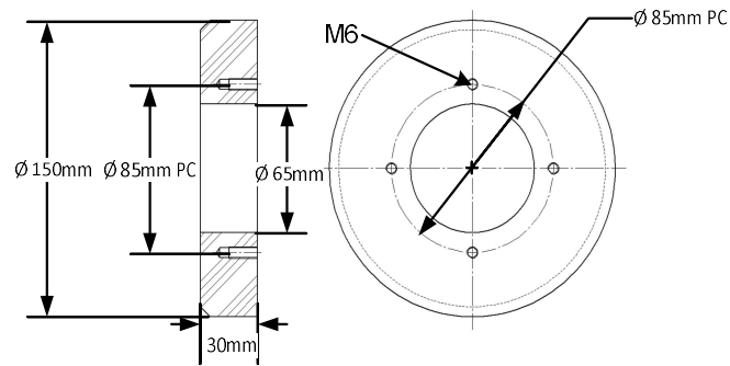
Figure 3: Mounting Boss
