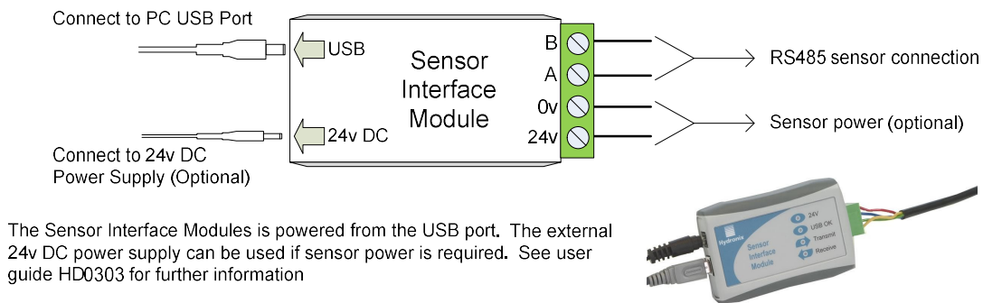
Figure 14: SIM01 USB-RS485 converter connections
