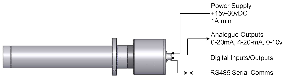
Figure 2: Connecting the sensor (overview)
