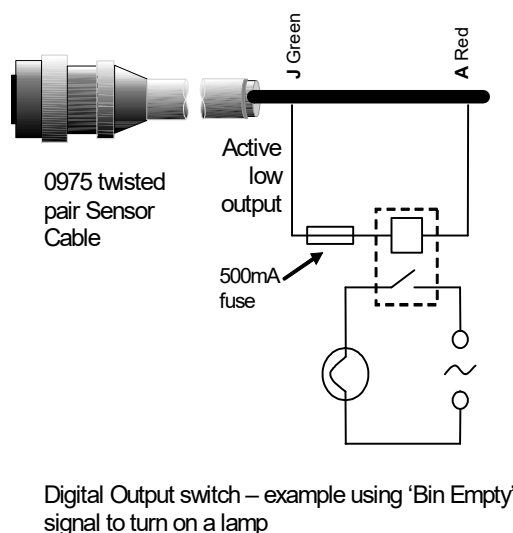
Figure 11: Activation of digital output 2
