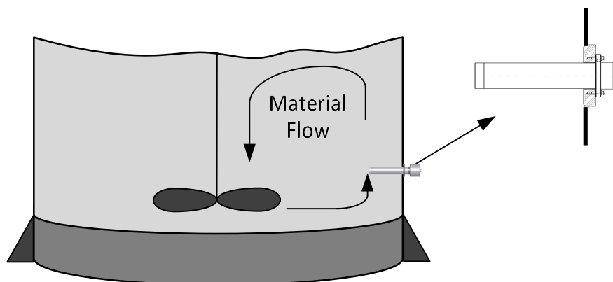
Figure 5: The sensor installed in a storage tank
