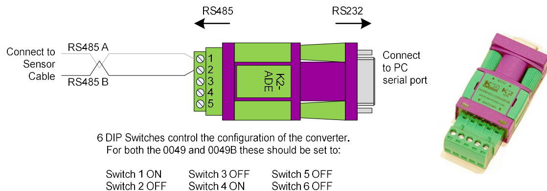
Figure 12: RS232/485 converter connections (0049B)
