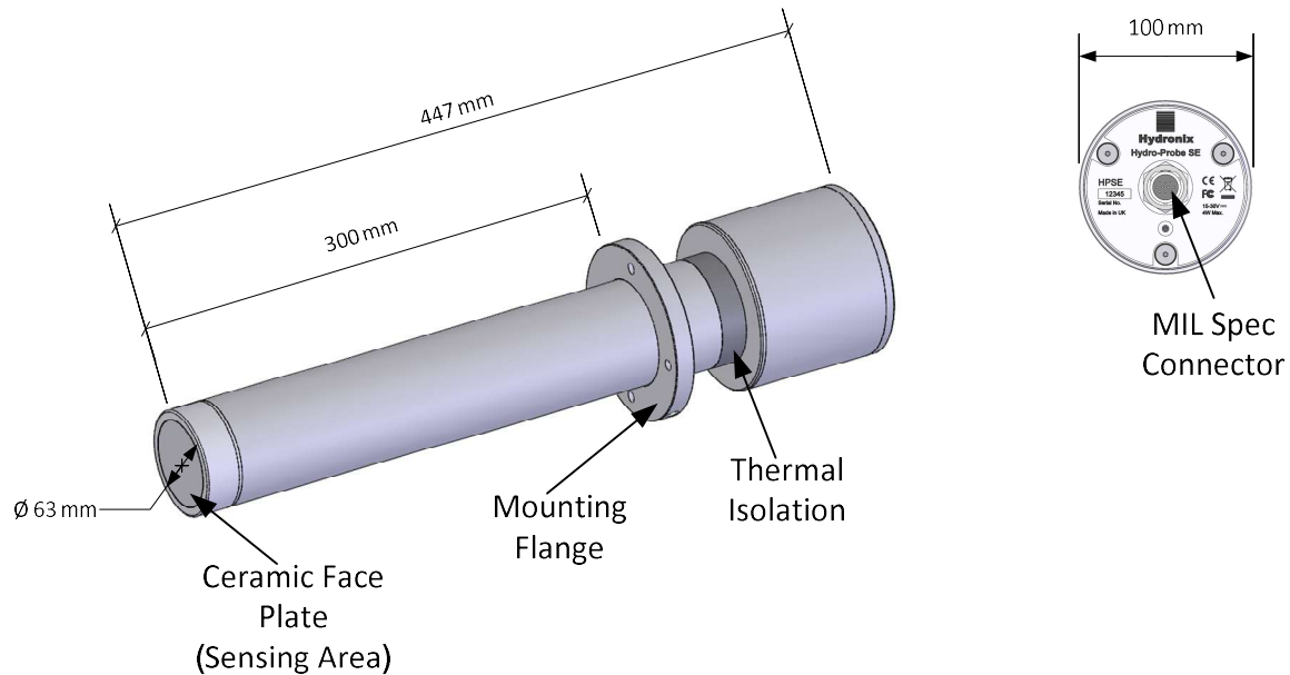
Figure 1: The Hydro-Probe SE
