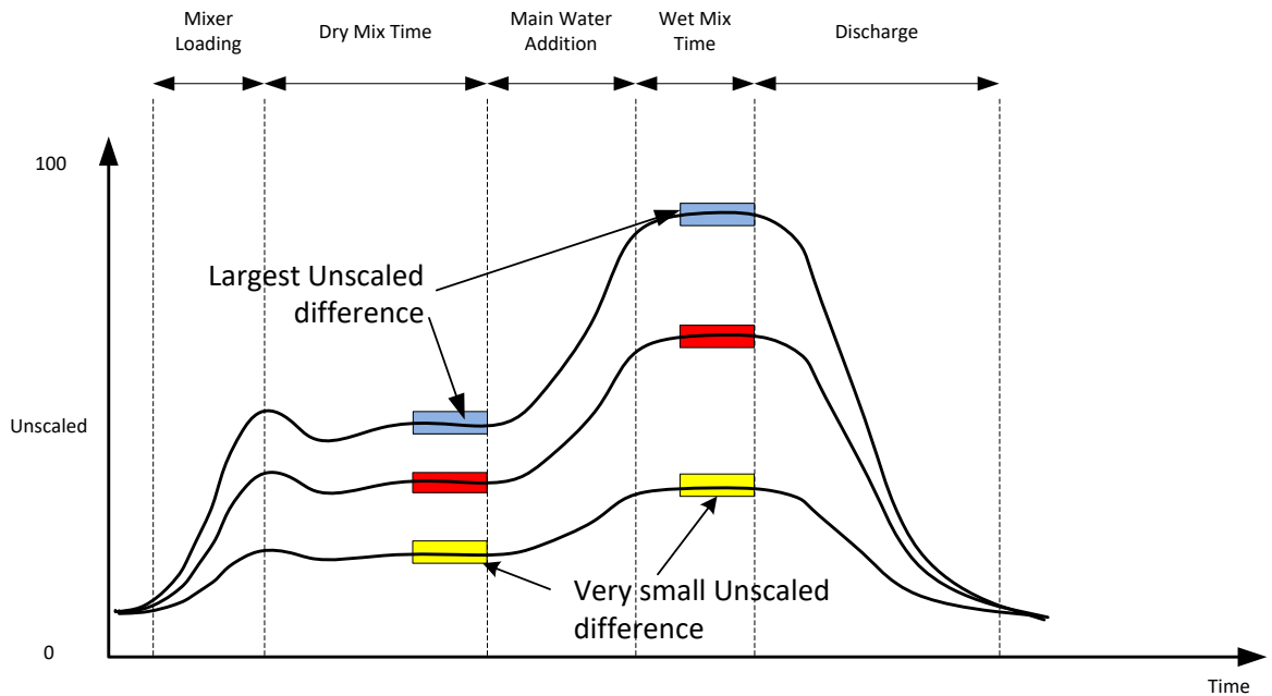
Figure 22: Comparing Measurement Modes
