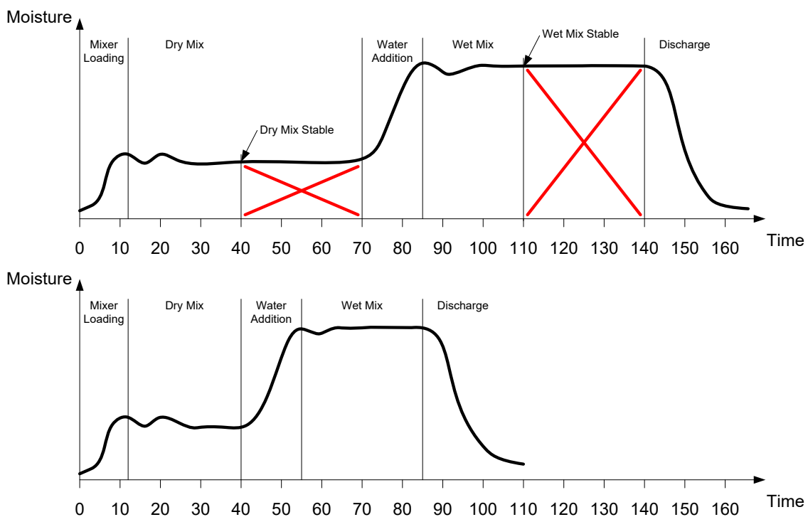
Figure 15: Extending the mix times for calibration
