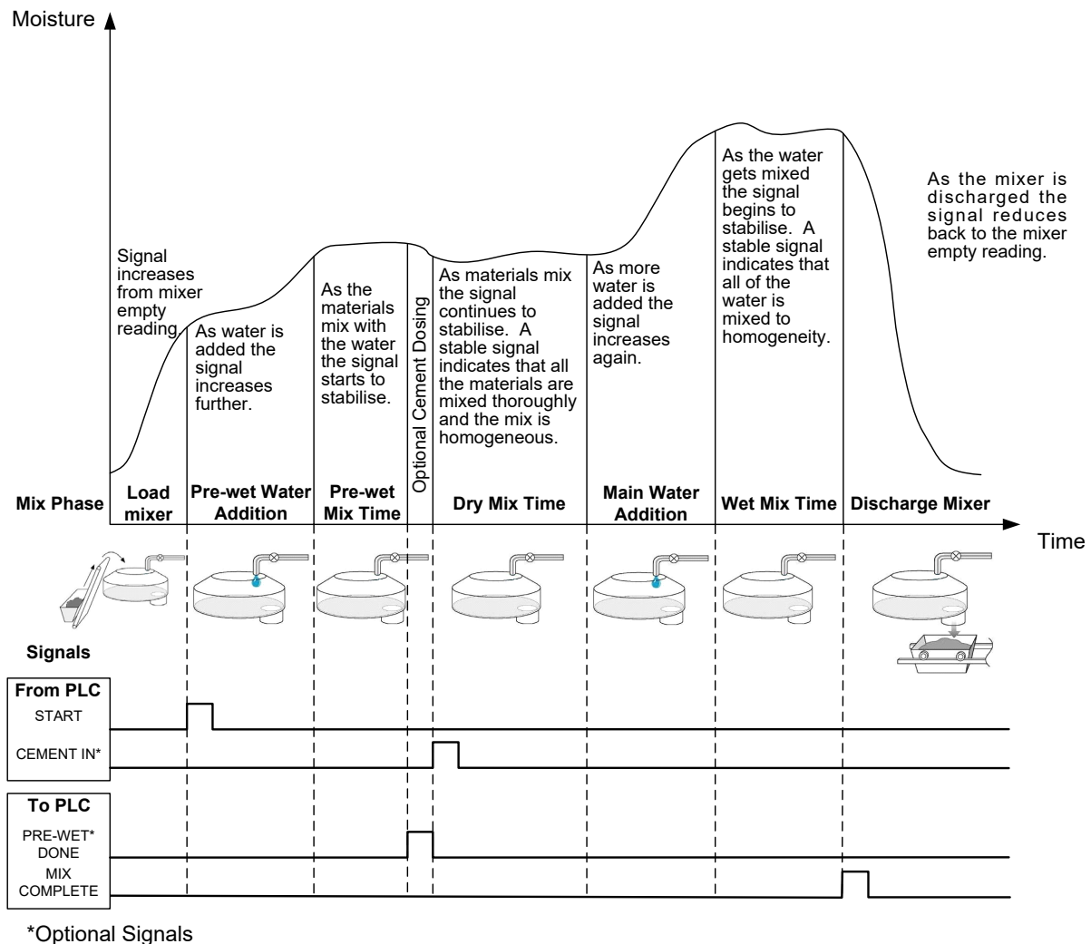
Figure 8: The mix cycle with pre-wet
