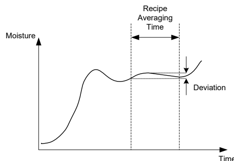
Figure 17: How the deviation is calculated
