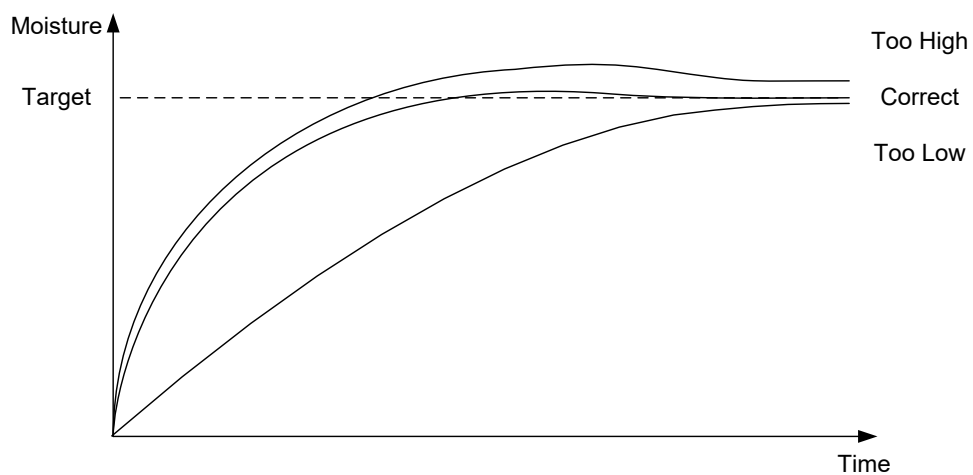
Figure 26: The effect of changing the Derivative Gain
