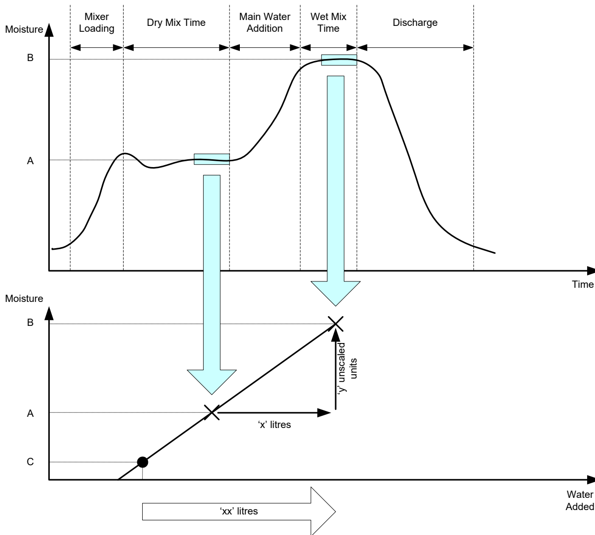
Figure 19: The CALC Mode Calculation
