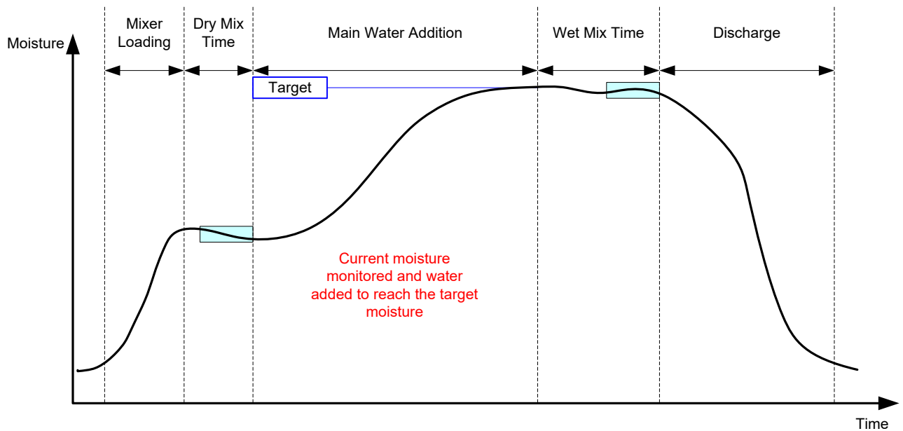
Figure 23: The moisture during AUTO Mode
