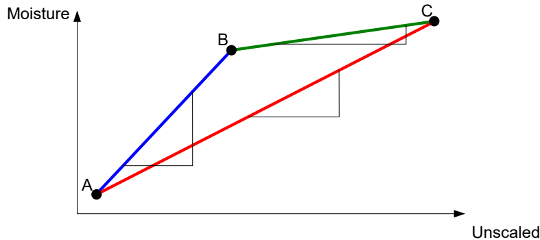
Figure 28: The calibration lines from the 2-step preset mode cycle
