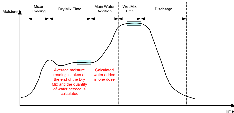
Figure 18: The moisture during CALC Mode
