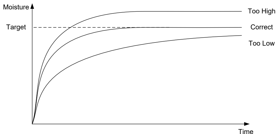
Figure 24: The effect of changing the Proportional Gain
