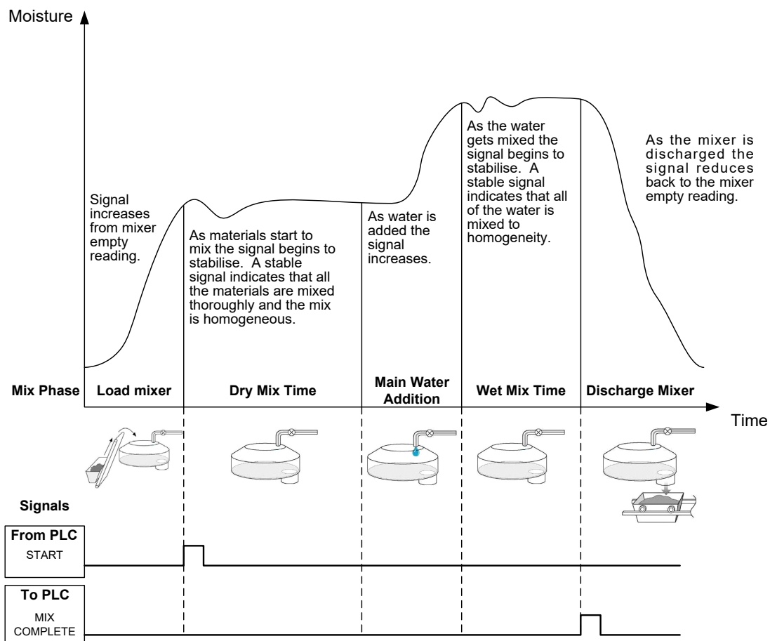
Figure 7: A simple mix cycle
