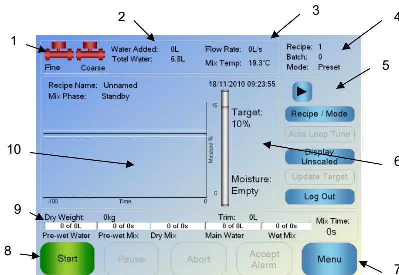
Figure 2: The Overview Screen of the Hydro-Control VI
