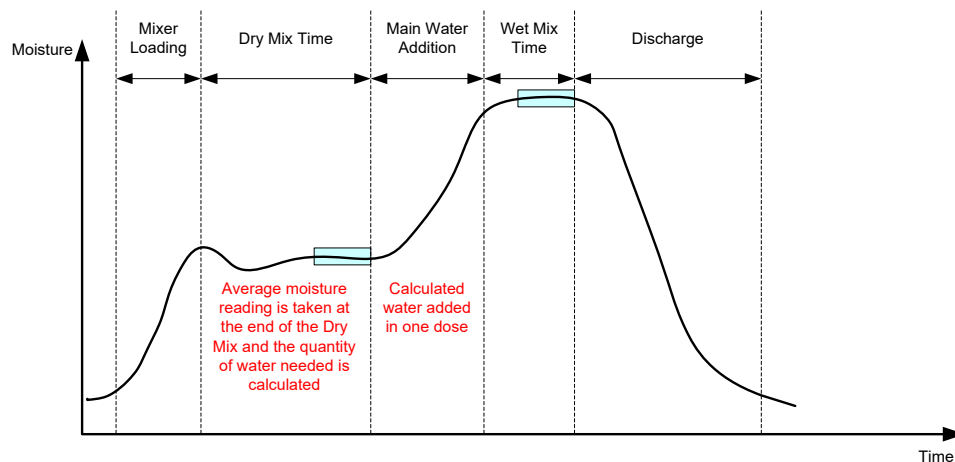
Figure 9: The moisture during CALC Mode
