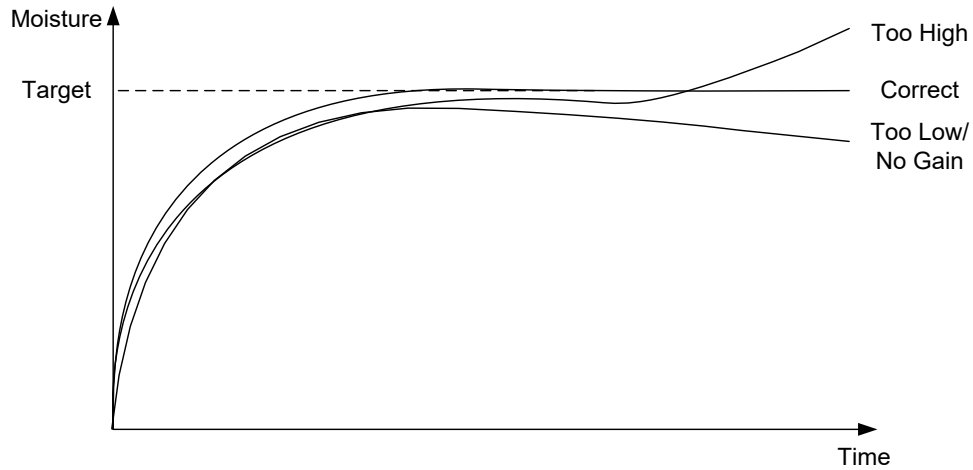
Figure 25: The effect of changing the Integral Gain
