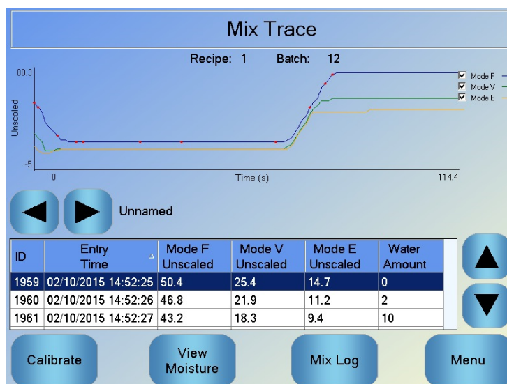
Figure 34: The Mix Trace Screen (Unscaled)
