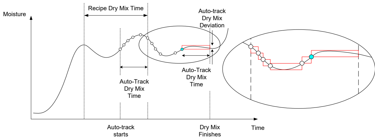
Figure 29: Mix trace showing the Auto-track function
