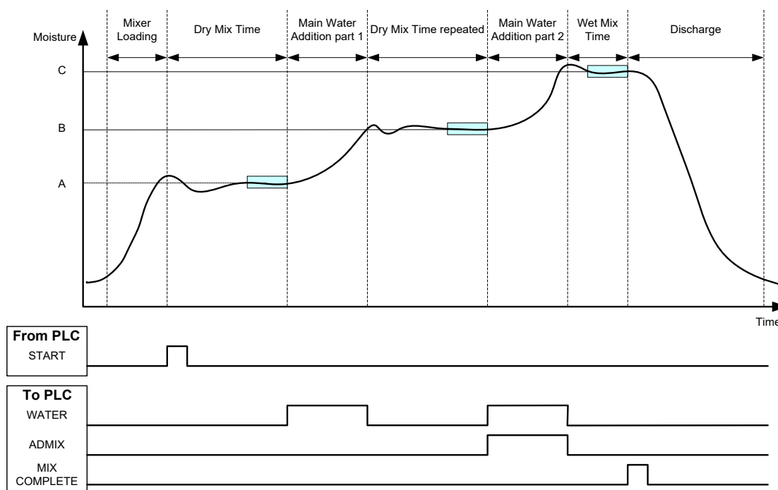
Figure 27: The 2 step preset mode cycle
