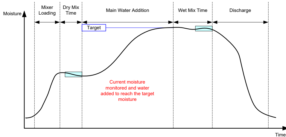
Figure 10: The moisture during AUTO Mode
