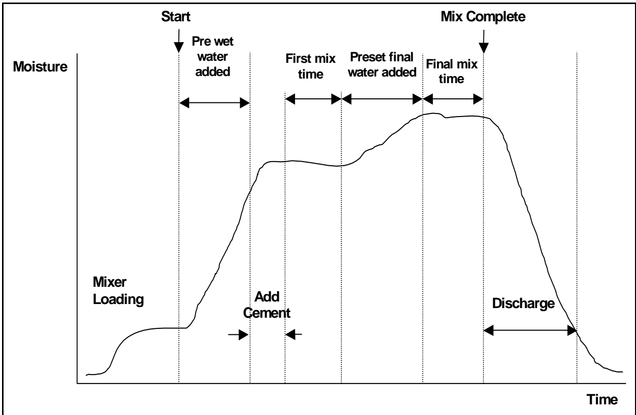
Figure 4 – Preset Mode Mix Cycle
