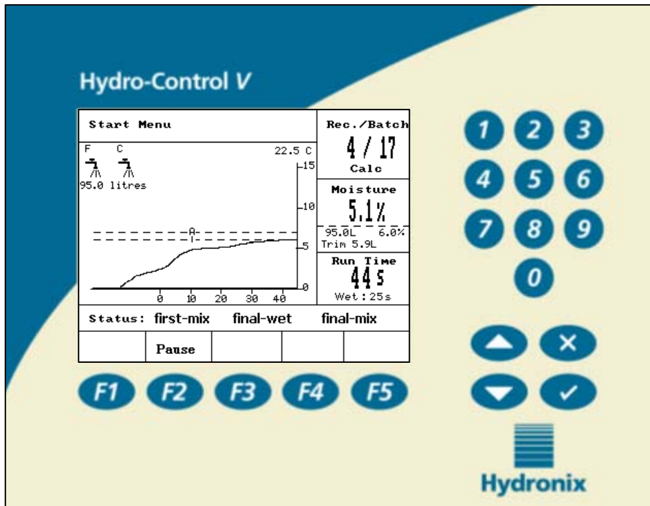
Figure 1 – Hydro-Control V - Front Panel
