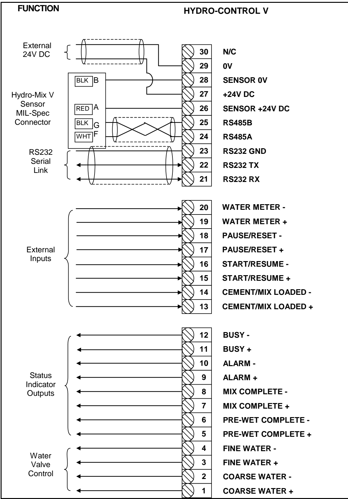
Figure 37 – System Interconnection
