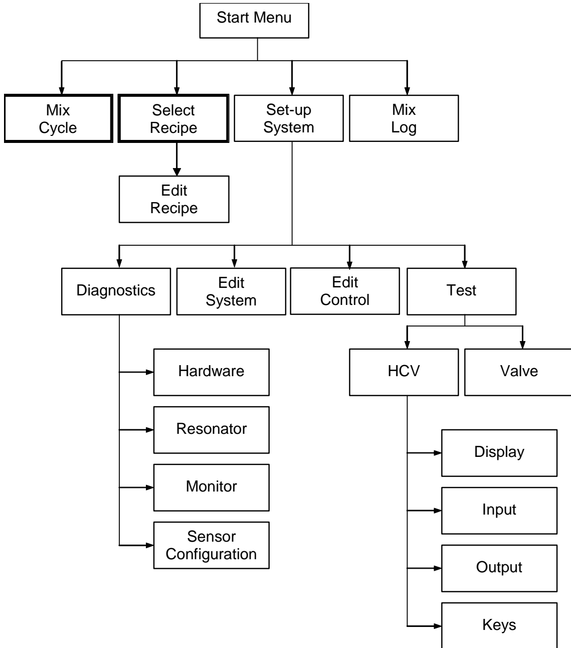
Figure 8 – Menu Tree
