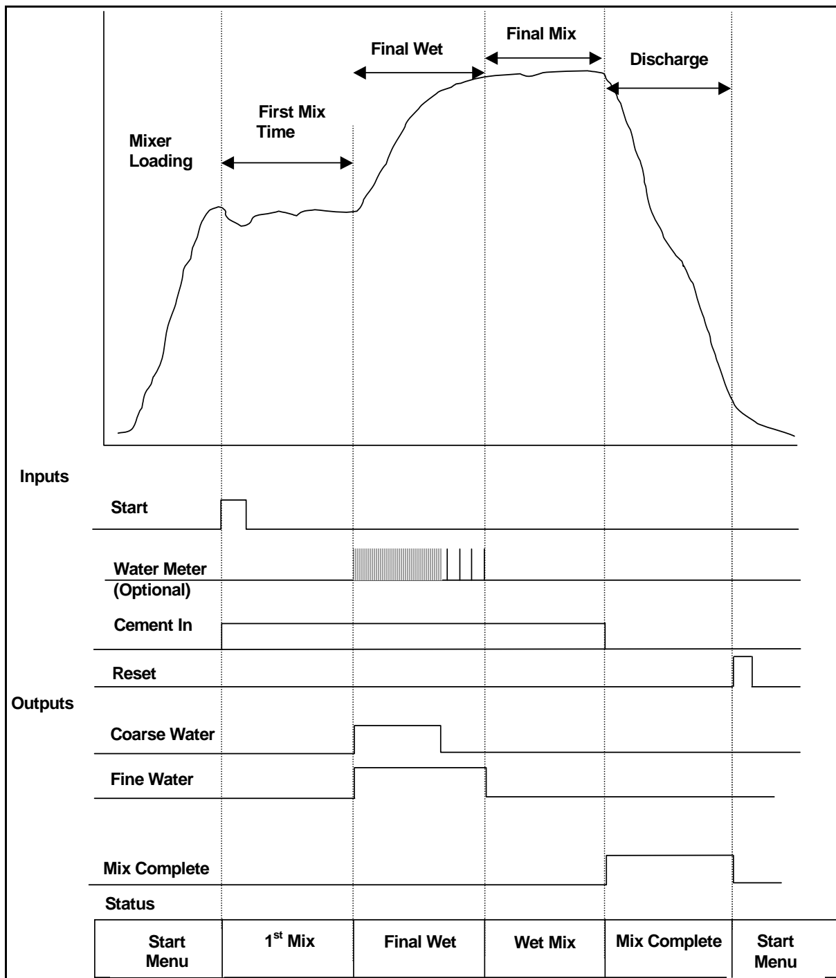
Figure 34 – Dry Mix Cycle (no Pre-Wet)
