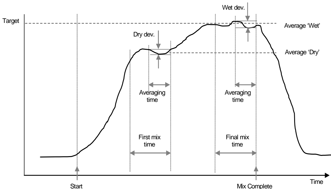
Figure 20 – Mix Log Deviations – Trend display
