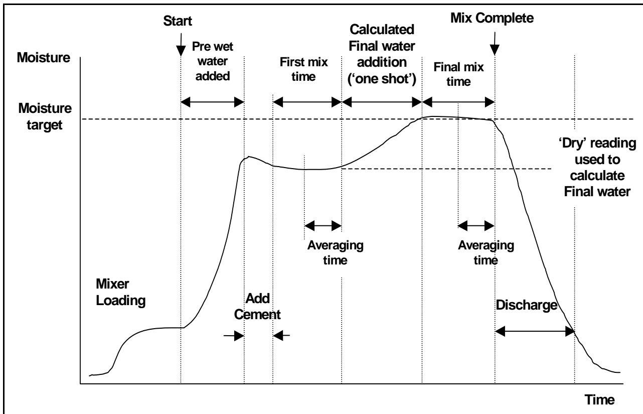
Figure 7 – Calc Mode Mix Cycle
