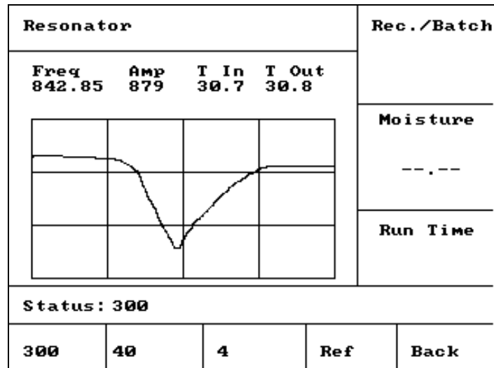
Figure 30 – Resonator
