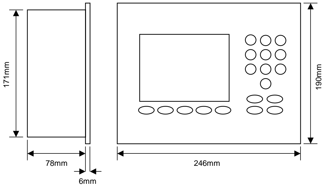
Figure 40 – Operator Panel Dimensions
