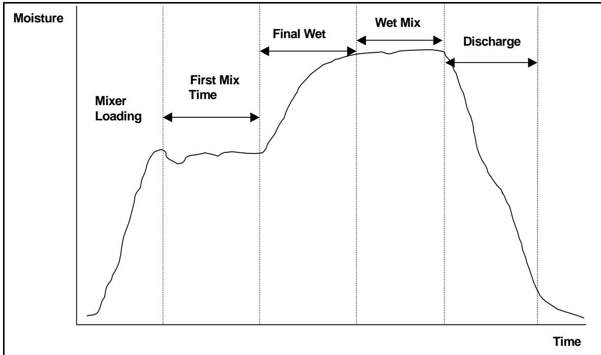
Figure 3 – 'Dry Mix' Mix Cycle
