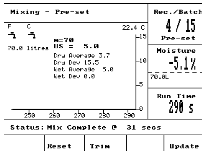
Figure 45 – Test mode screen
