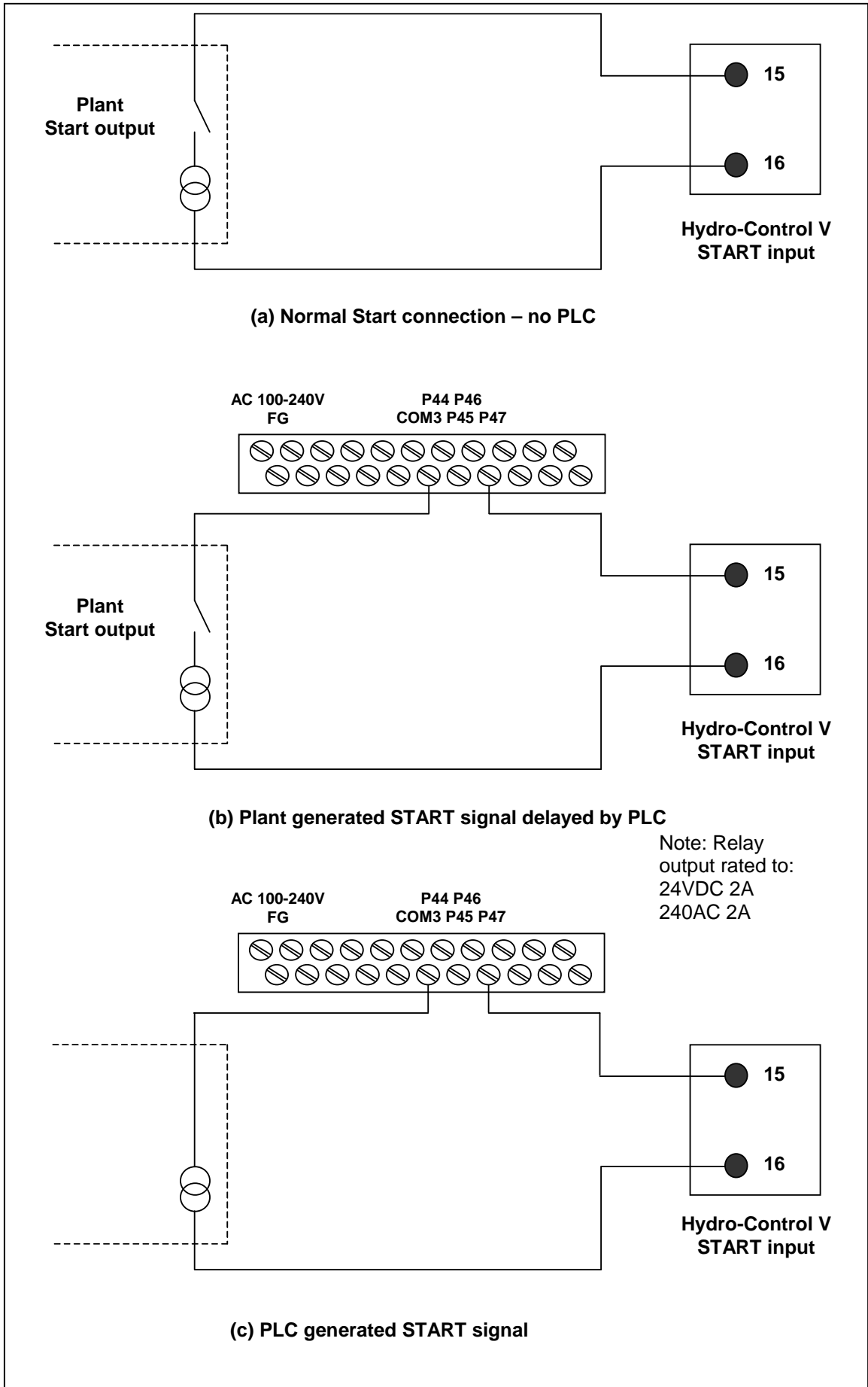
Figure 42 – Remote Recipe PLC Start Signal Options
