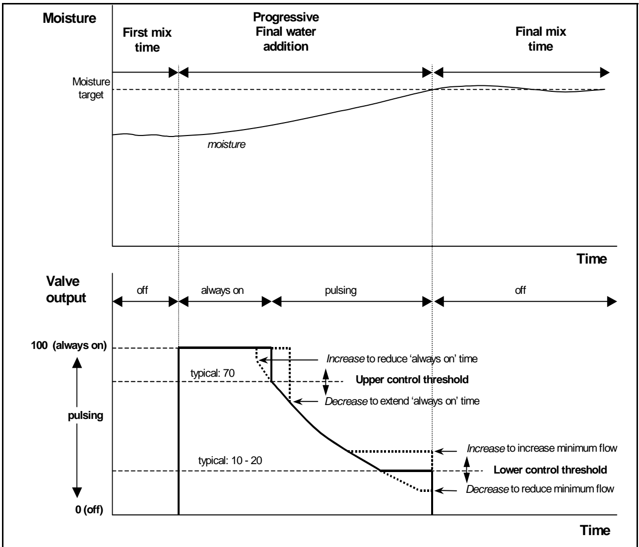
Figure 6 – Valve Control in Auto Mode
