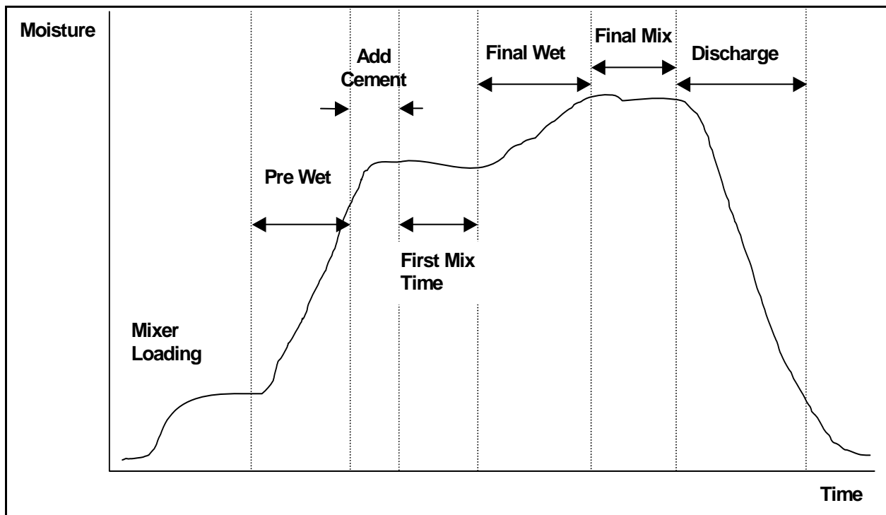
Figure 2 – 'Pre-Wet' Mix Cycle
