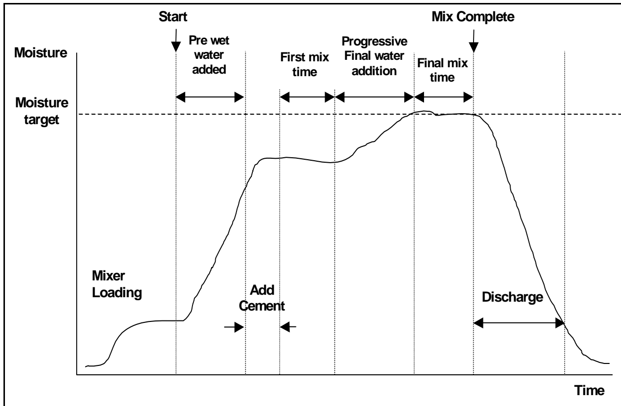
Figure 5 – Auto Mode Mix Cycle
