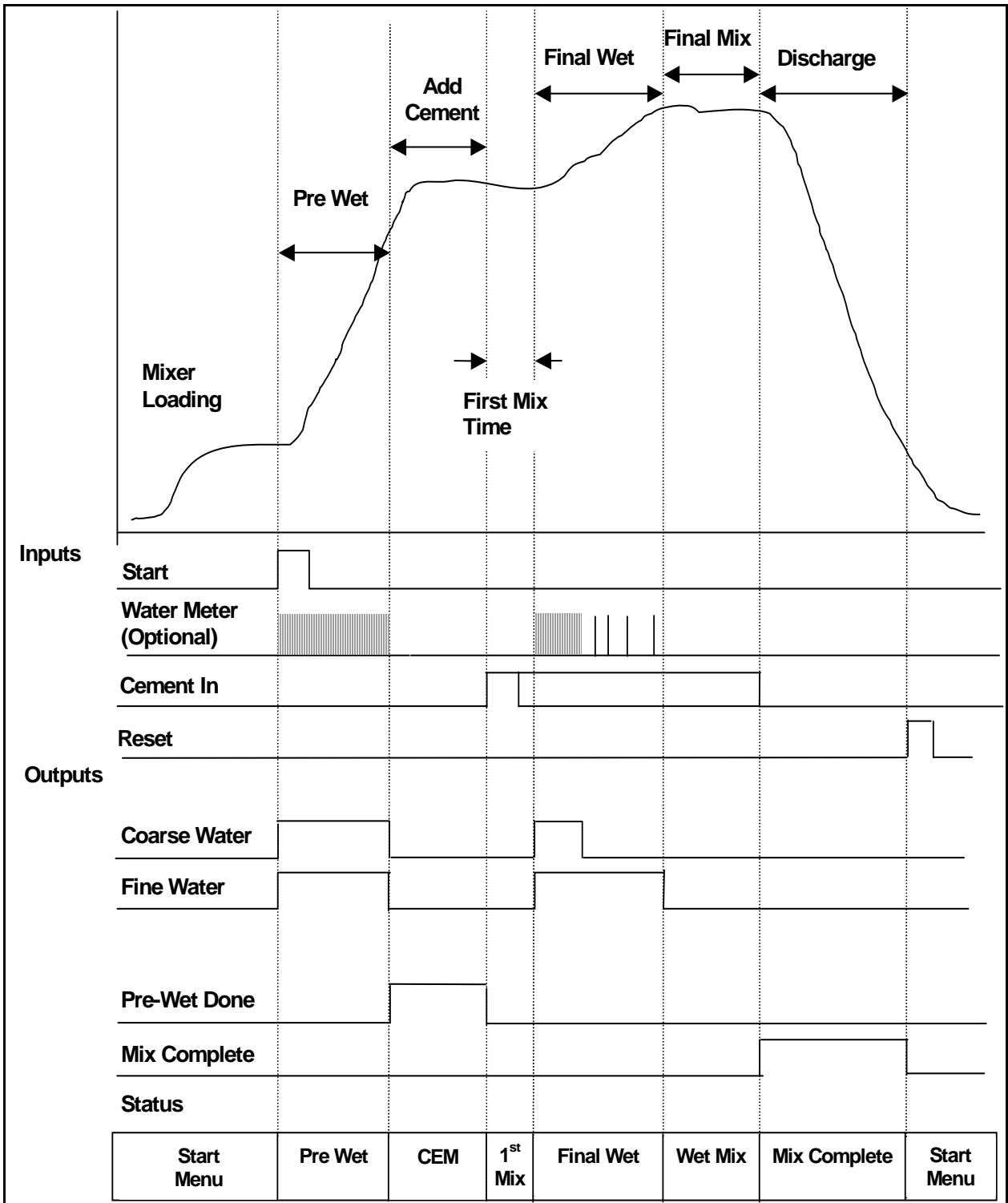
Figure 33 – Pre-Wet Mix Cycle
