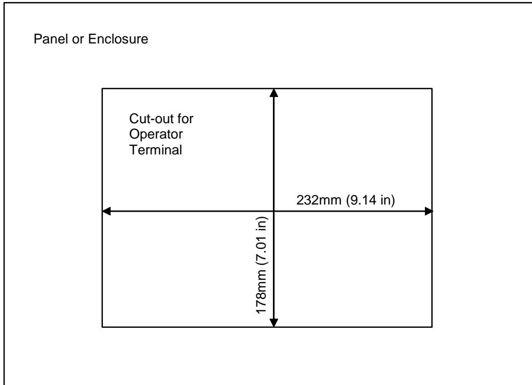
Figure 39 – Panel cut-out for Operator Terminal
