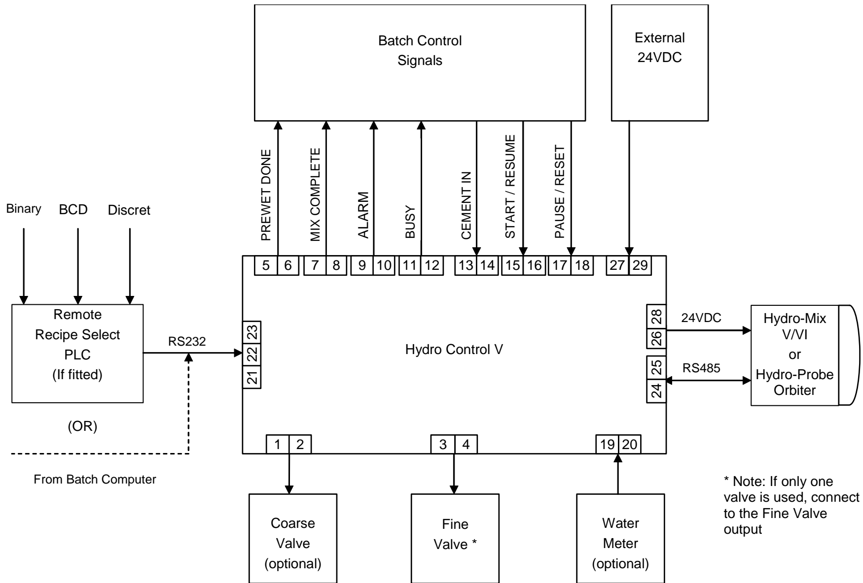
Figure 36 – System Block Diagram
